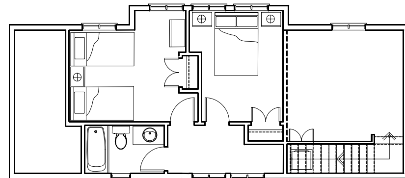
SECOND FLOOR
